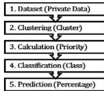
Gambar 1. Framework
